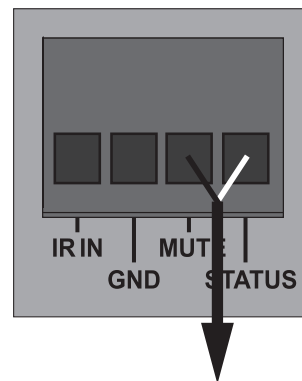
To +V/GND on Voltage Controlled Device Zone Voltage Control Connection
