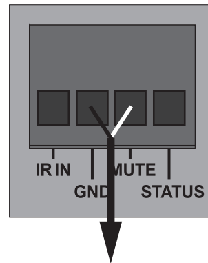
To +V/GND on Trigger Device Zone Mute Connection
