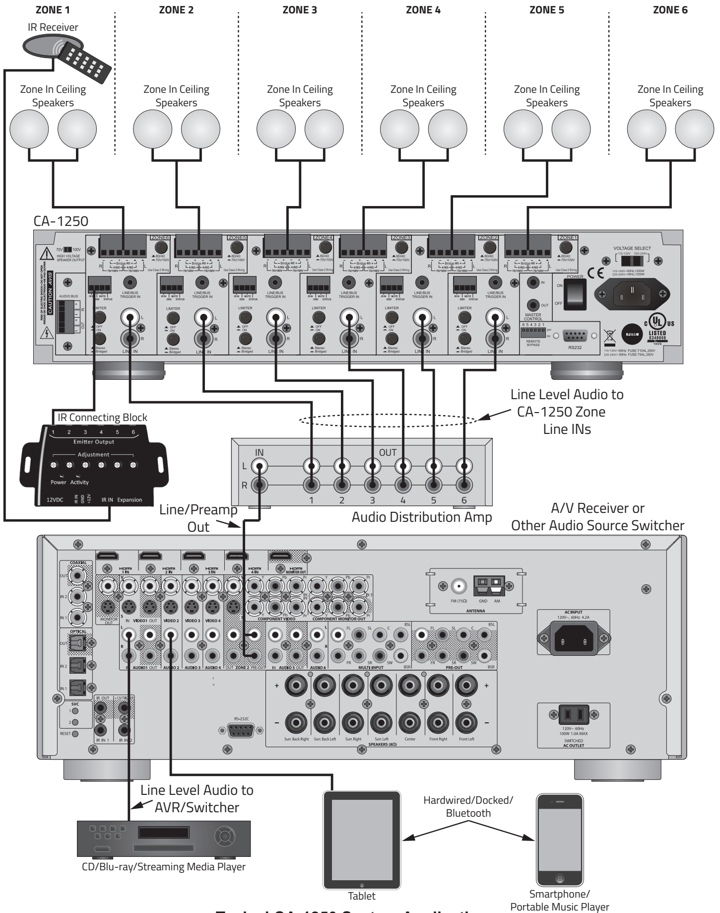
Typical CA-1250 System Application
