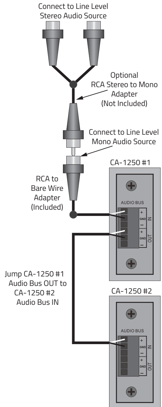
Audio Bus IN/OUT Connections
