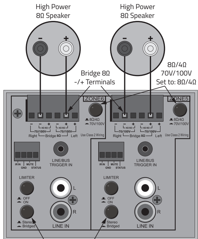
Stereo/Bridged Set to: Bridged Bridged 8Ω Connection
