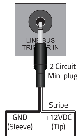
Zone Line/Bus Trigger Connection
